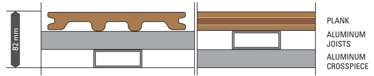
LAYING ON ALUMINUM JOISTS AND CROSSPIECES 40 x 30 mm (W x H) WITH SUPERIMPOSED FRAME
